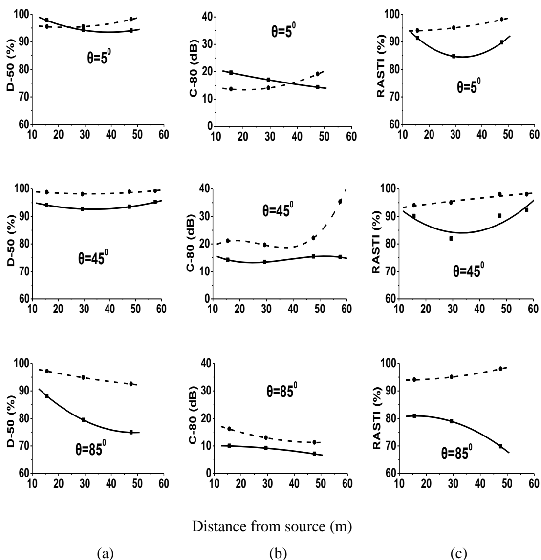
Figure 6 - (a) Definition D-50, (b) Clarity C-80, (c) Speech Intelligibility RASTI, as function of receiver distance and angle from the source (in the centre of the stage). The results are from -- measurements and from --- simulations [ ].
